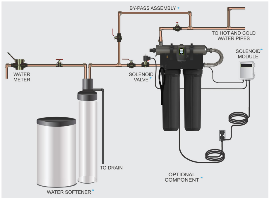
Figure 1. Typical Installation
