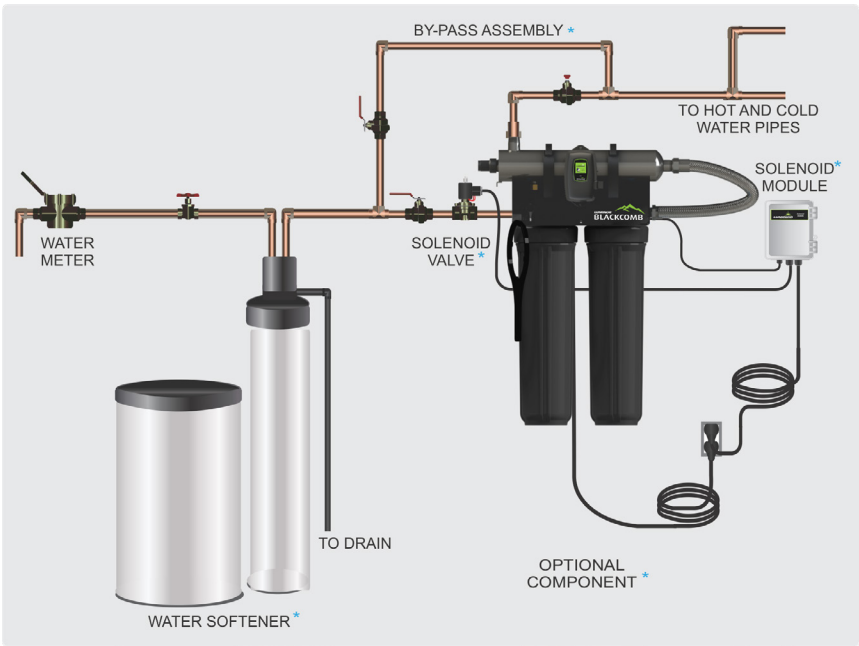
Figure 1. Typical Installation
